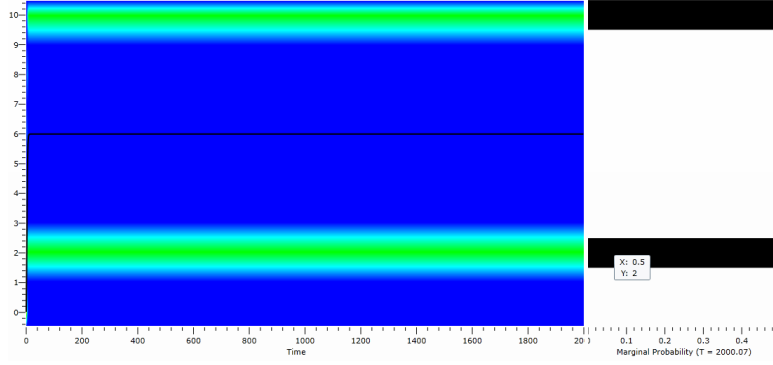
Fig. 4: The figure plots the CME solution for species \lambda_{out} . Vertical axes represent the number of molecules of \lambda_{out} , while horizontal axes represent time or marginal probability of molecules of \lambda_{out}
