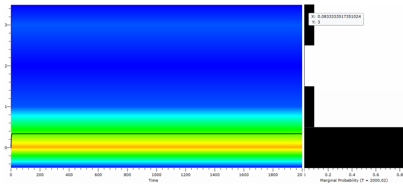
Fig. 3: The figure plots the CME solution for species \lambda_{out} . Vertical axes represent the number of molecules of \lambda_{out} , while horizontal axes represent time or marginal probability of molecules of species \lambda_{out}
