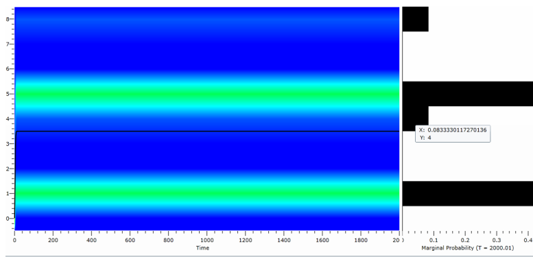
Fig. 2: The figure plots the CME solution for the species \lambda_{out} . Vertical axes represent the number of molecules of \lambda_{out} , while horizontal axes represent time or marginal probability of molecules of species \lambda_{out}
