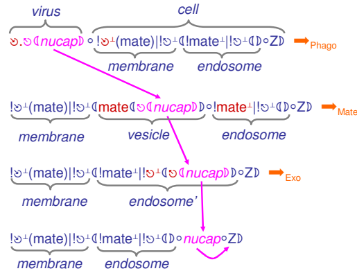
Figure 7 Viral Infection
