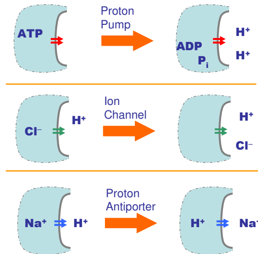
Figure 10 Molecular Channels
