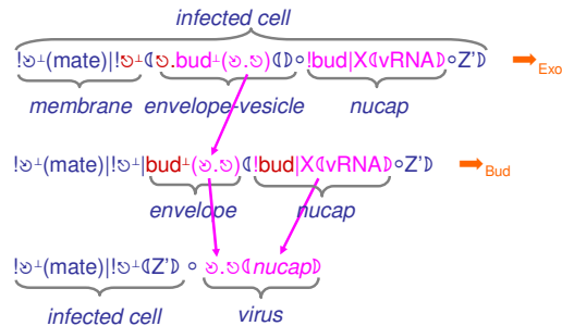
Figure 8 Viral Reproduction
