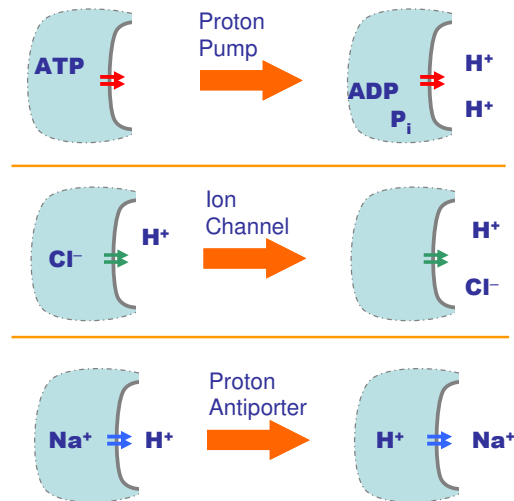
Figure 10 Molecular Channels
