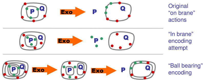
Figure 13 Exo Encodings
