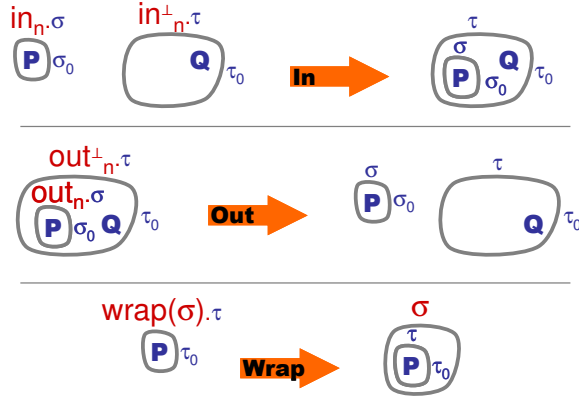
Figure 12 Atonal Reactions
